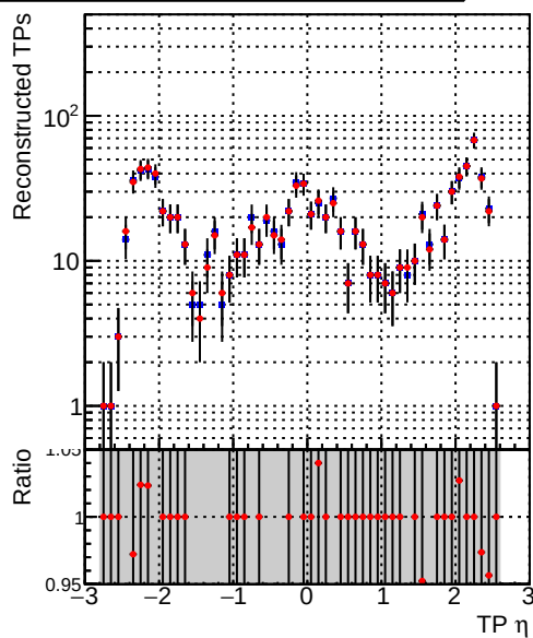
N of simulated tracks vs TP \eta N of associated tracks (simToReco) vs TP \eta
