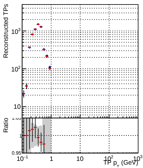
Legend: DQM_CKF_TTbase (blue line with dots), DQM_CKF_TT_retrainOldFiles125_v2_prelimWPM_epoch1 (red line with dots)
