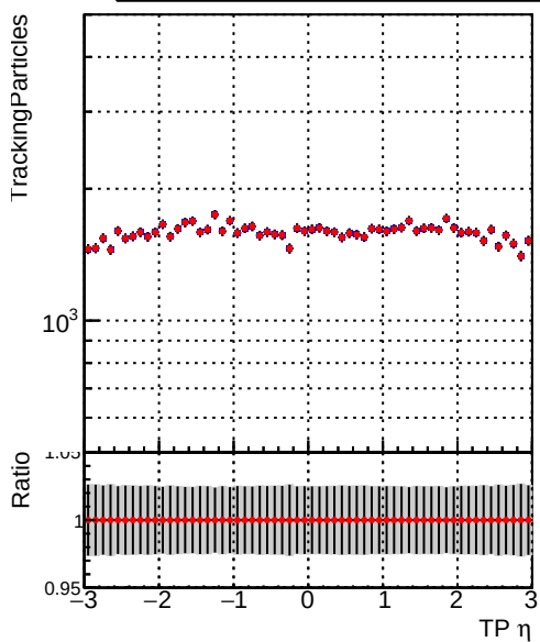
■ DQM_CKF_TTbase ● DQM_CKF_TT_retrainOldFiles125_v2_prelimWPM_epoch1
