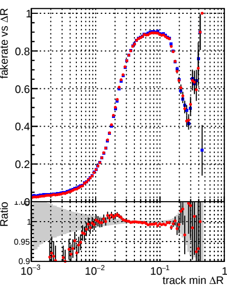
Legend: DQM_CKF_TTbase (blue line with points), DQM_CKF_TT_retrainOldFiles125_v2_prelimWPM_epoch1 (red line with points)
