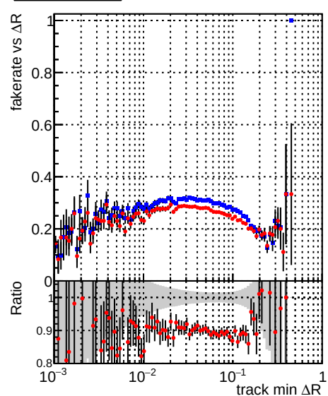
Fake rate vs \Delta R (track, jet) Legend: DQM_CKF_TTbase DQM_CKF_TT_retrainOldFiles125_v2_prelimWPM_epoch1
