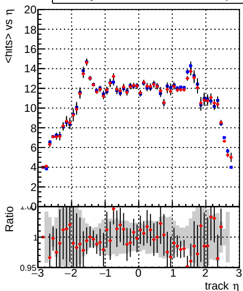
mean hits vs \eta Legend: DQM_CKF_TTbase (blue line), DQM_CKF_TT_retrainOldFiles125_v2_prelimWPM_epoch1 (red line)
