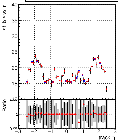
— DQM_CKF_TTbase — DQM_CKF_TT_retrainOldFiles125_v2_prelimWPM_epoch1
