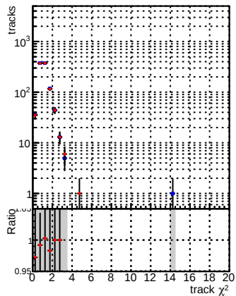
N of reco track vs. \chi^2 for DQM_CKF_TTbase (blue) and DQM_CKF_TT_retrainOldFiles125_v2_prelimWPM_epoch1 (red)
