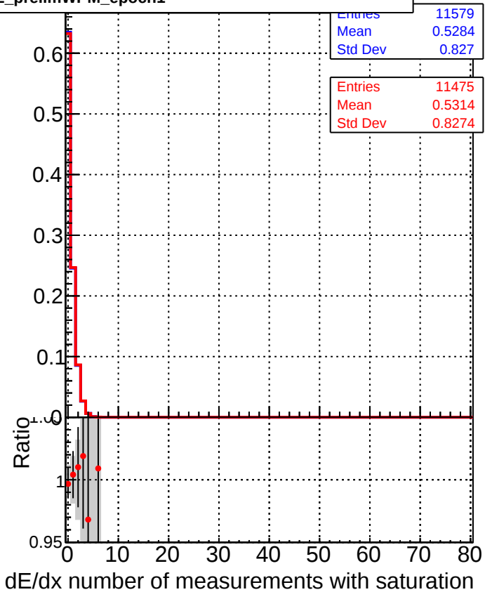
■ DQM_CKF_TTbase ● DQM_CKF_TT_retrainOldFiles125_v2_prelimWPM_epoch1
