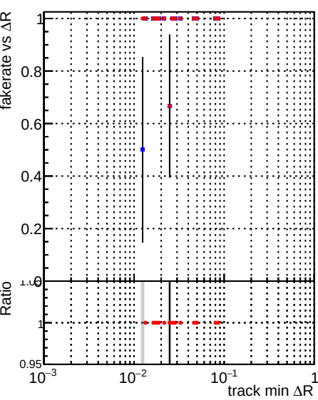
Legend: DQM_CKF_TTbase (grey bars), DQM_CKF_TT_retrainOldFiles125_v2_prelimWPM_epoch1 (red dots with error bars)
