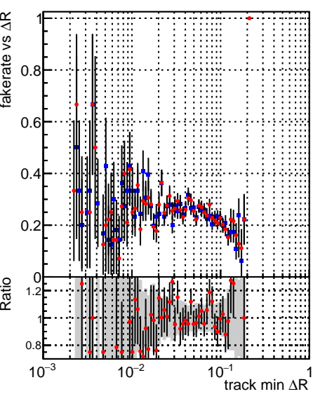
—●— DQM_CKF_TTbase —●— DQM_CKF_TT_retrainOldFiles125_v2_prelimWPM_epoch1
