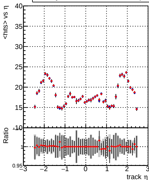
mean hits vs \eta Legend: — DQM_CKF_TTbase — DQM_CKF_TT_retrainOldFiles125_v2_prelimWPM_epoch1
