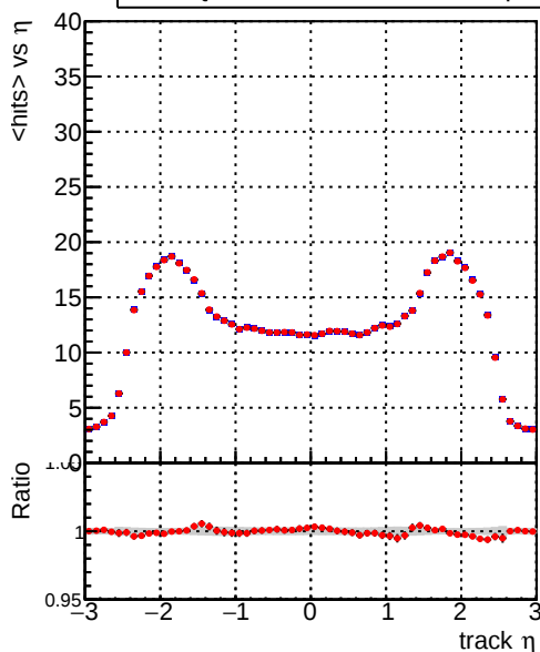
— DQM_CKF_TTbase — DQM_CKF_TT_retrainOldFiles125_v2_prelimWPM_epoch1
