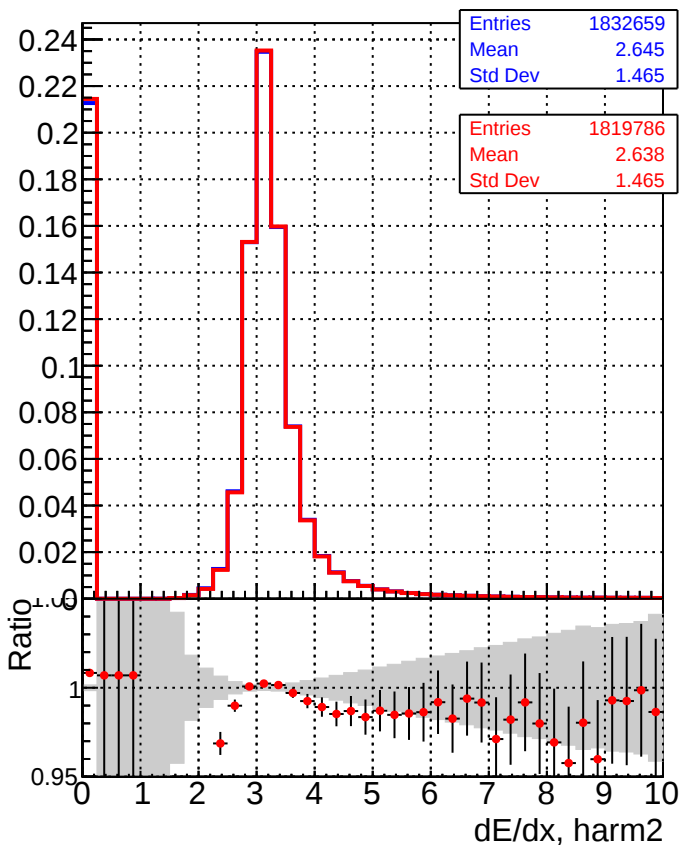
—■— DQM_CKF_TTbase —●— DQM_CKF_TT_retrainOldFiles125_v2_prelimWPM_epoch1
