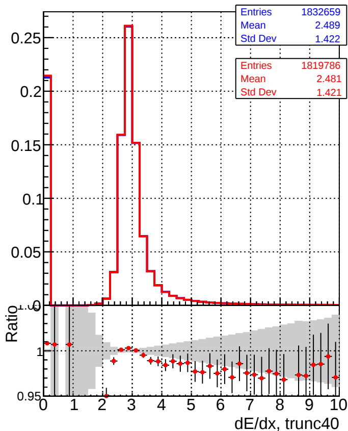
—■— DQM_CKF_TTbase —●— DQM_CKF_TT_retrainOldFiles125_v2_prelimWPM_epoch1
