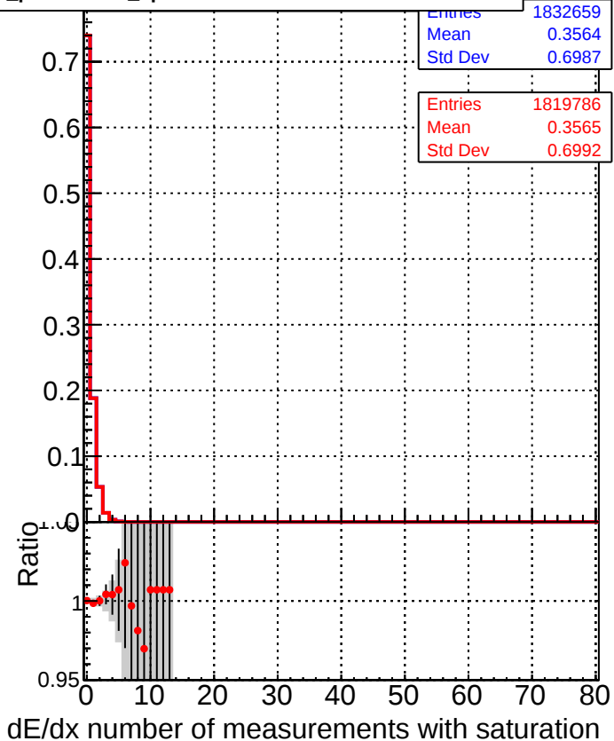
—■— DQM_CKF_TTbase —●— DQM_CKF_TT_retrainOldFiles125_v2_prelimWPM_epoch1
