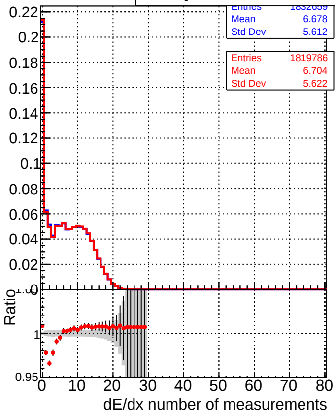
—■— DQM_CKF_TTbase —●— DQM_CKF_TT_retrainOldFiles125_v2_prelimWPM_epoch1
