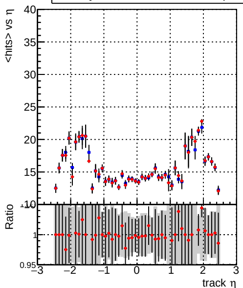
mean hits vs \eta — DQM_CKF_TTbase — DQM_CKF_TT_retrainOldFiles125_v2_prelimWPM_epoch1
