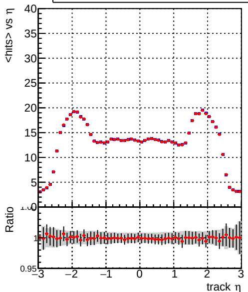
mean hits — DQM_CKF_TTbase — DQM_CKF_TT_retrainOldFiles125_v2_prelimWPM_epoch1
