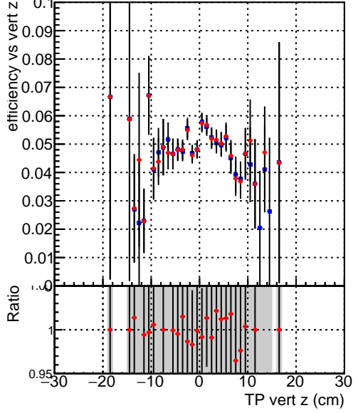
Efficiency vs. TP vert z (left) and fake+duplicates vs. track ref. point z (right). Legend: DQM_CKF_TTbase (blue squares), DQM_CKF_TT_retrainOldFiles125_v2_prelimWPM_epoch1 (red circles).
