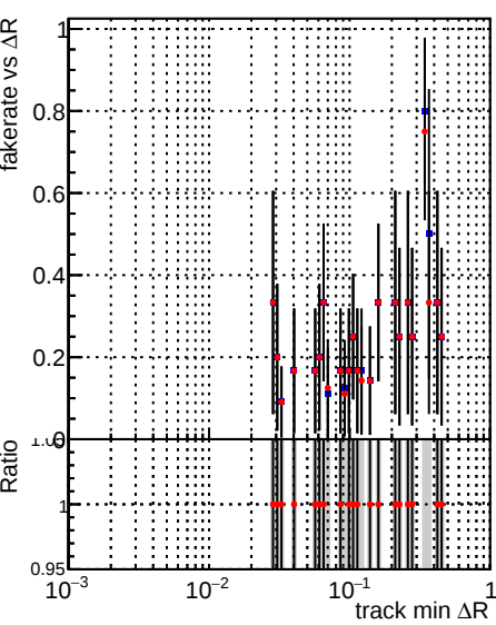
Legend: DQM_CKF_TTbase (blue dots), DQM_CKF_TT_retrainOldFiles125_v2_prelimWPM_epoch1 (red dots)
