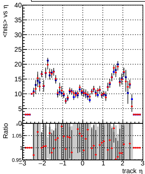
mean hits vs \eta Legend: DQM_CKF_TTbase (blue line with error bars), DQM_CKF_TT_retrainOldFiles125_v2_prelimWPM_epoch1 (red line with error bars)
