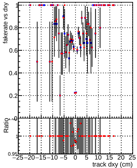
—●— DQM_CKF_TTbase —●— DQM_CKF_TT_retrainOldFiles125_v2_prelimWPM_epoch1
