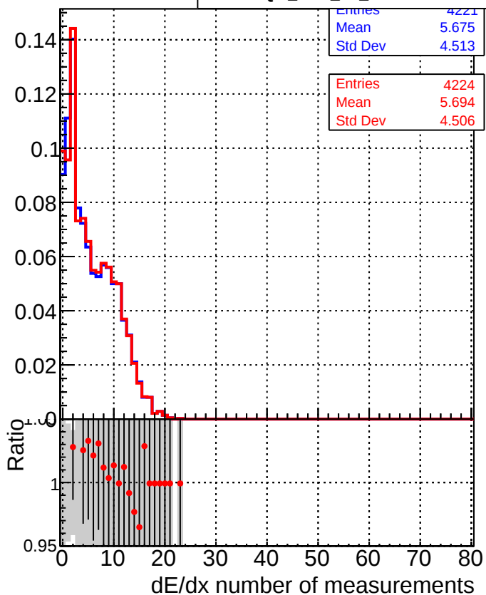
DQM_CKF_TTbase DQM_CKF_TT_retrainOldFiles125_v2_prelimWPM_epoch1
