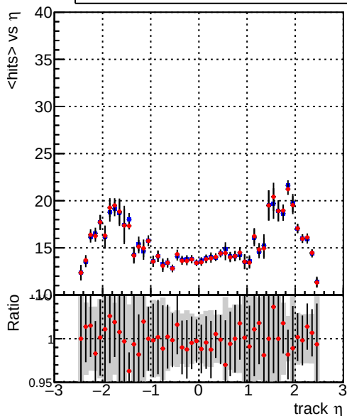
mean hit — DQM_CKF_TTbase — DQM_CKF_TT_retrainOldFiles125_v2_prelimWPM_epoch1
