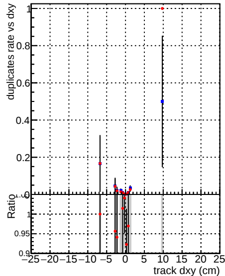
—●— DQM_CKF_TTbase —●— DQM_CKF_TT_retrainOldFiles125_v2_prelimWPM_epoch1
