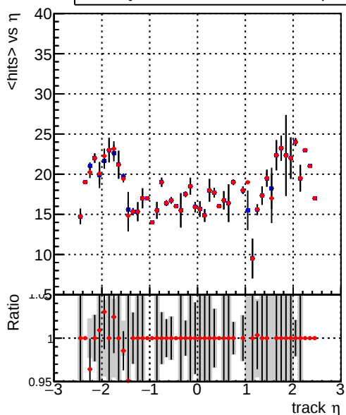
mean hit Legend: DQM_CKF_TTbase (blue line with dots), DQM_CKF_TT_retrainOldFiles125_v2_prelimWPM_epoch1 (red line with dots)
