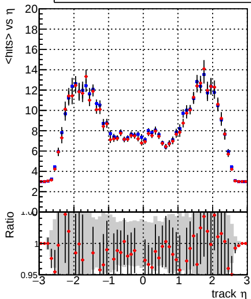
mean hits vs \eta Legend: DQM_CKF_TTbase (blue line with dots), DQM_CKF_TT_retrainOldFiles125_v2_prelimWPM_epoch1 (red line with dots)
