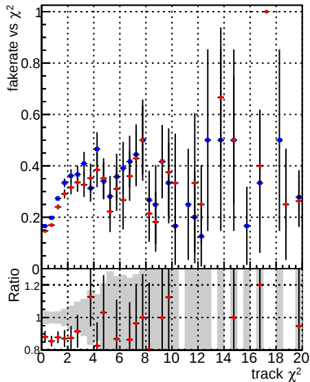
Fake rate vs. —•— DQM_CKF_TTbase —•— DQM_CKF_TT_retrainOldFiles125_v2_prelimWPM_epoch1
