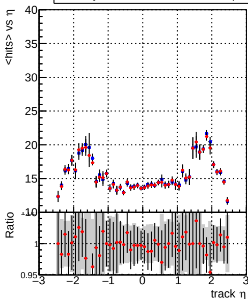
mean hits vs \eta Legend: DQM_CKF_TTbase (blue line with markers), DQM_CKF_TT_retrainOldFiles125_v2_prelimWPM_epoch1 (red line with markers)
