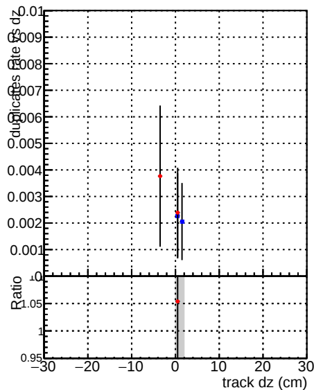
—●— DQM_CKF_TTbase —●— DQM_CKF_TT_retrainOldFiles125_v2_prelimWPM_epoch1
