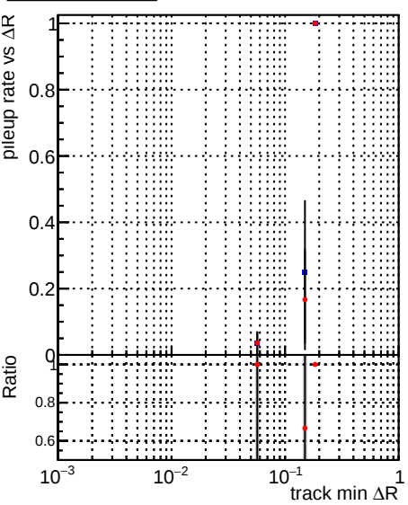
Legend: DQM_CKF_TTbase (blue), DQM_CKF_TT_retrainOldFiles125_v2_prelimWPM_epoch1 (red)
