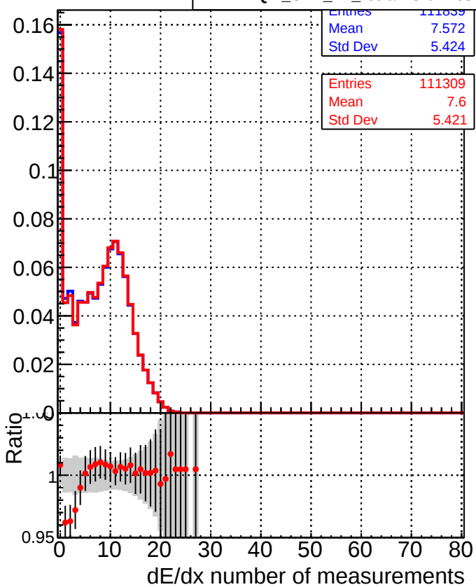
■ DQM_CKF_TTbase ● DQM_CKF_TT_retrainOldFiles125_v2_prelimWPM_epoch1
