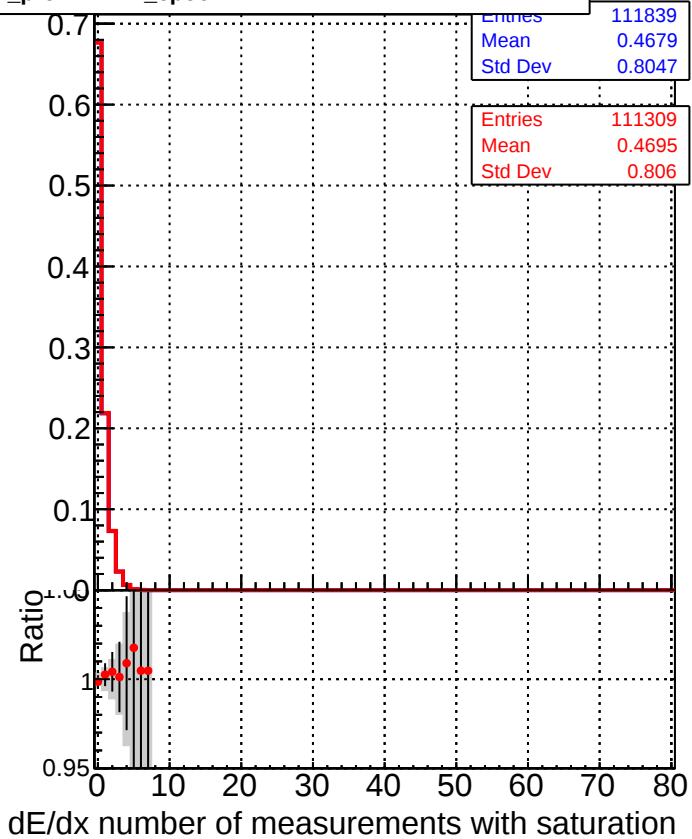
■ DQM_CKF_TTbase ● DQM_CKF_TT_retrainOldFiles125_v2_prelimWPM_epoch1
