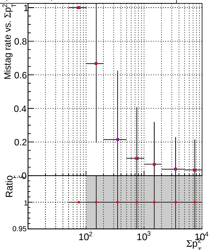
—•— DQM_CKF_TTbase —•— DQM_CKF_TT_retrainOldFiles125_v2_prelimWPM_epoch1
