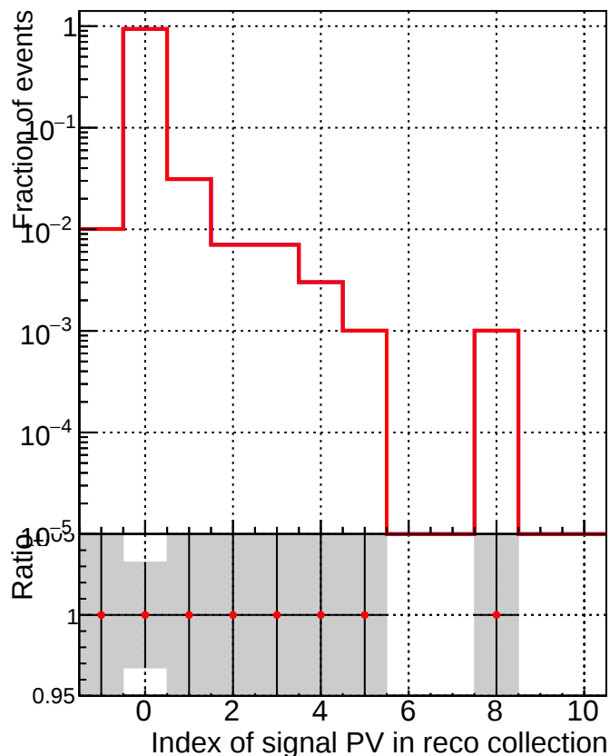
—•— DQM_CKF_TTbase —•— DQM_CKF_TT_retrainOldFiles125_v2_prelimWPM_epoch1
