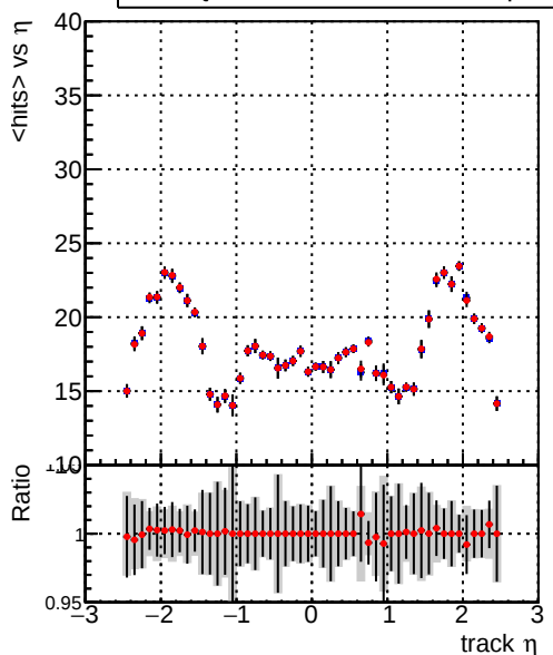
mean hits vs \eta Legend: DQM_CKF_TTbase (blue line), DQM_CKF_TT_retrainOldFiles125_v2_prelimWPM_epoch1 (red line)
