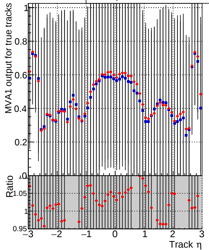
MVA1 of associated tracks (recoToSim) vs. track \eta Legend: ■ DQM_CKF_TTbase ◆ DQM_CKF_TT_retrainOldFiles125_v2_prelimWPM_epoch1
