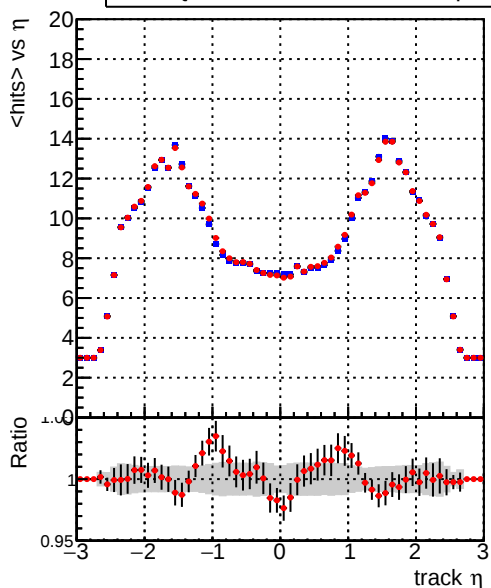
— DQM_CKF_TTbase — DQM_CKF_TT_retrainOldFiles125_v2_prelimWPM_epoch1
