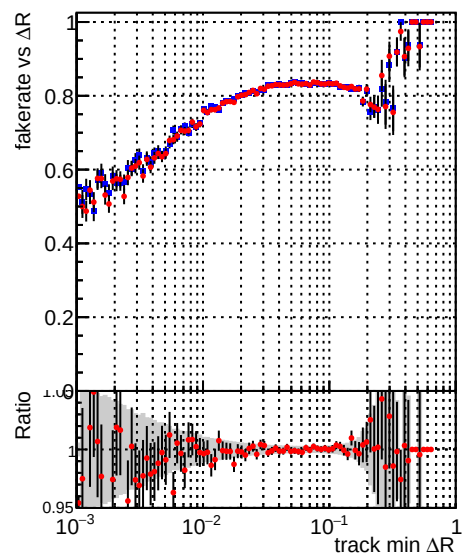
—●— DQM_CKF_TTbase —●— DQM_CKF_TT_retrainOldFiles125_v2_prelimWPM_epoch1
