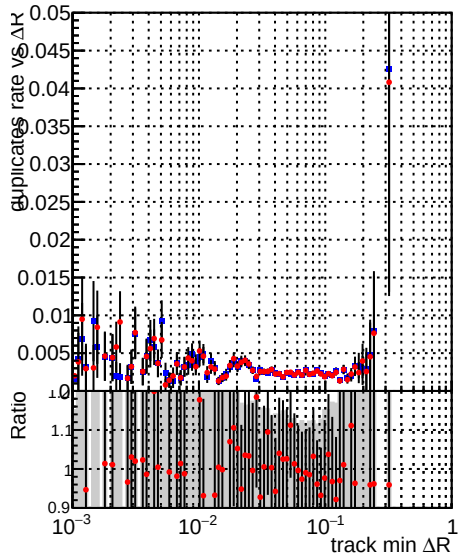
—●— DQM_CKF_TTbase —●— DQM_CKF_TT_retrainOldFiles125_v2_prelimWPM_epoch1
