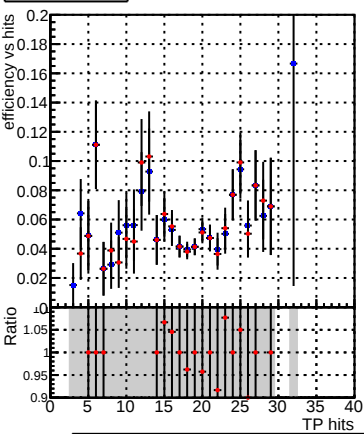
Efficiency vs hit Legend: DQM_CKF_TTbase (blue diamond), DQM_CKF_TT_retrainOldFiles125_v2_prelimWPM_epoch1 (red cross)
