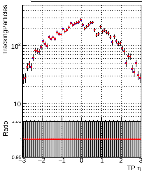
N of simulated tracks vs TP \eta Legend: DQM_CKF_TTbase (blue line), DQM_CKF_TT_retrainOldFiles125_v2_prelimWPM_epoch1 (red line)
