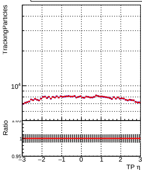
N of simulated tracks vs \eta Legend: DQM_CKF_TTbase (blue dots), DQM_CKF_TT_retrainOldFiles125_v2_prelimWPM_epoch1 (red dots)
