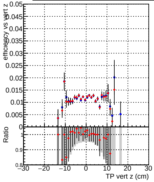
Efficiency vs. TP vert z — DQM_CKF_TTbase — DQM_CKF_TT_retrainOldFiles125_v2_prelimWPM_epoch1
