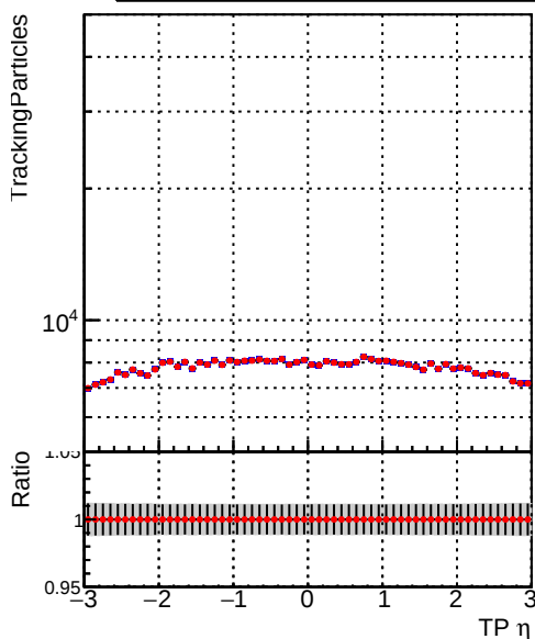
—•— DQM_CKF_TTbase —•— DQM_CKF_TT_retrainOldFiles125_v2_prelimWPM_epoch1
