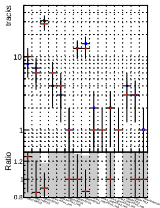
N of reco track vs. \chi^2 —●— DQM_CKF_TTbase —●— DQM_CKF_TT_retrainOldFiles125_v2_prelimWPM_epoch1
