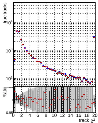
N of reco track vs. \chi^2 for DQM CKF TTbase and DQM CKF TT_retrainOldFiles125_v2_prelimWPM_epoch1
