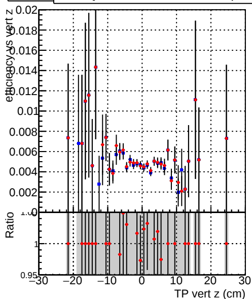
Efficiency vs. TP vert z (cm) — DQM_CKF_TTbase — DQM_CKF_TT_retrainOldFiles125_v2_prelimWPM_epoch1
