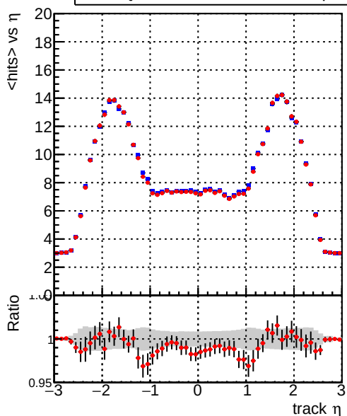
mean hits vs \eta — DQM_CKF_TTbase — DQM_CKF_TT_retrainOldFiles125_v2_prelimWPM_epoch1
