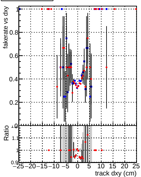
—■— DQM_CKF_TTbase —●— DQM_CKF_TT_retrainOldFiles125_v2_prelimWPM_epoch1
