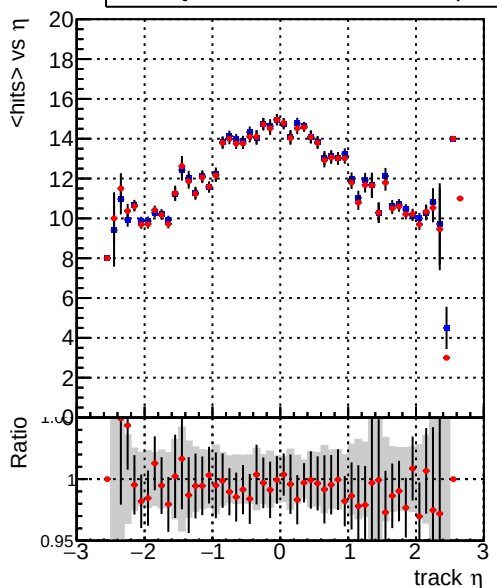
— DQM_CKF_TTbase — DQM_CKF_TT_retrainOldFiles125_v2_prelimWPM_epoch1 mean hits vs \eta
