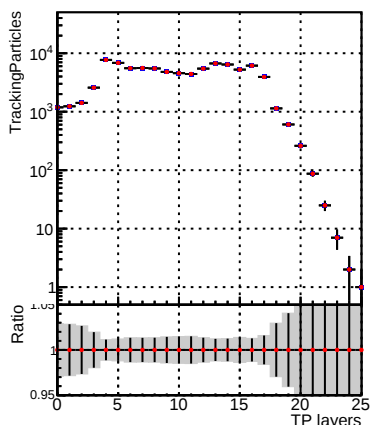
N of sim DQM_CKF_TT_retrainOldFiles125_v2_prelimWPM_epoch0
