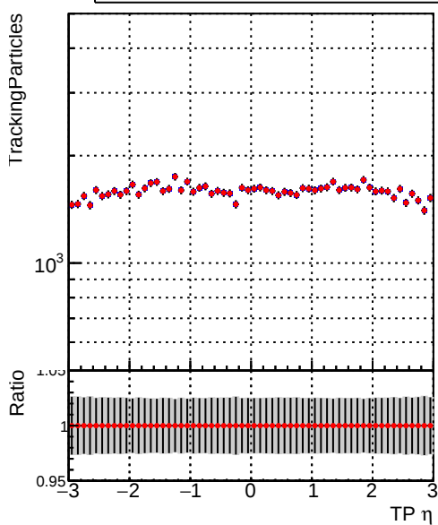
N of simulated tracks vs \eta Legend: DQM_CKF_TTbase (blue line with dots), DQM_CKF_TT_retrainOldFiles125_v2_prelimWPM_epoch0 (red line with dots)
