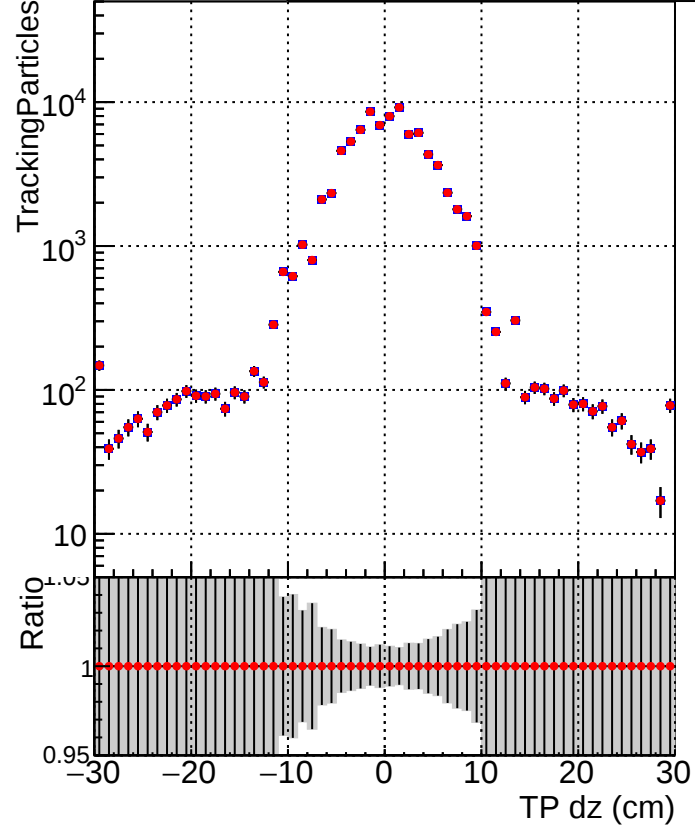
N of simulated track Legend: DQM_CKF_TTbase DQM_CKF_TT_retrainOldFiles125_v2_prelimWPM_epoch0
