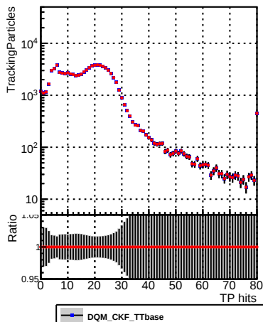
N of sim DQM_CKF_TTbase DQM_CKF_TT_retrainOldFiles125_v2_prelimWPM_epoch0
